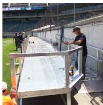
Individual platform components were manufactured in AAE's shop and delivered for on-site install
